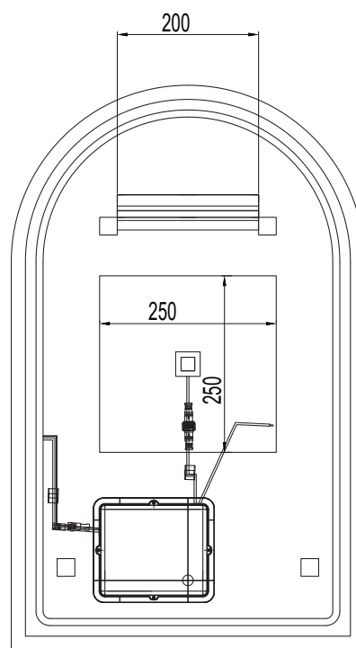
BACK VIEW
